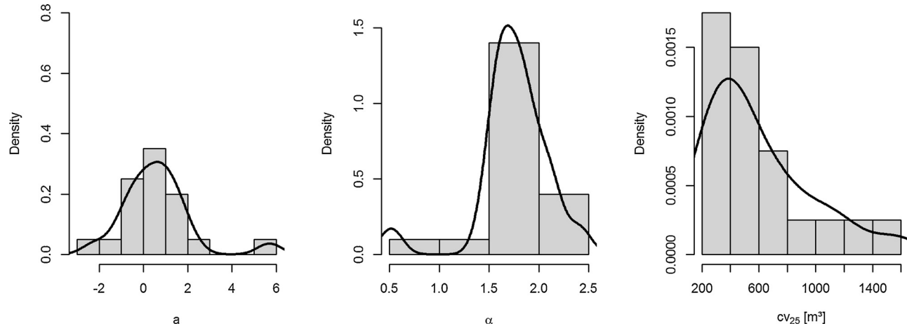
Fig. 9. Histograms and empirical density functions of the species specific parameter estimates (95% quantile regression) a (left) and α (middle) in the allometric relationship \ln(\text{cv}) = a + \alpha \times \ln(d) (Eq. (5)). The rightmost histogram shows the distribution of the estimated crown volumes cv 25 which result for d = 25 cm.
