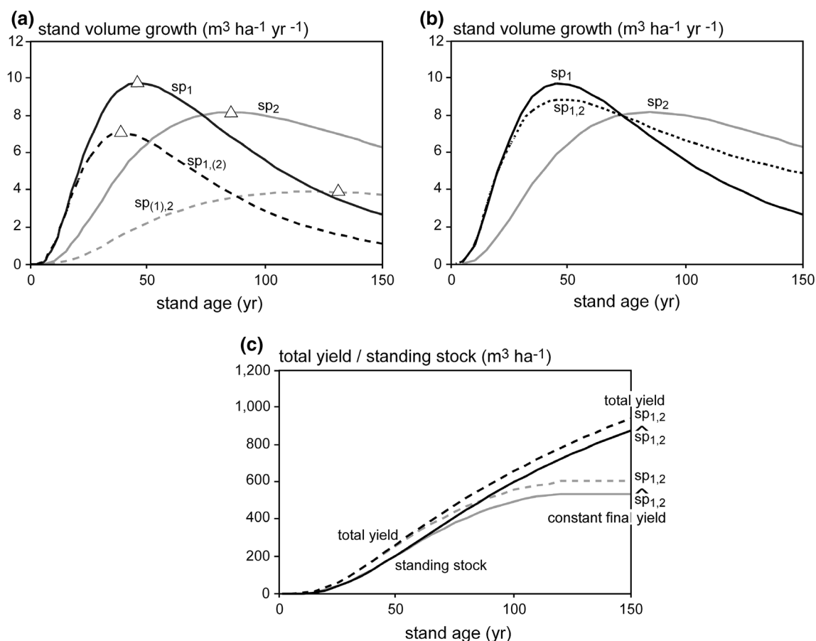
Fig. 4 Mixing can modulate the course of stand growth, yield, and standing stock: a course of annual volume growth in pure stands ( \text{sp}_1 and \text{sp}_2 ) and of both species in a mixed stand ( \text{sp}_{1,2} ) and \hat{\text{sp}}_{1,2} ; see notation in Table 4; triangle the level and the age of culmination; b the course of total stand growth in mixed ( \text{sp}_{1,2} ) compared with pure
